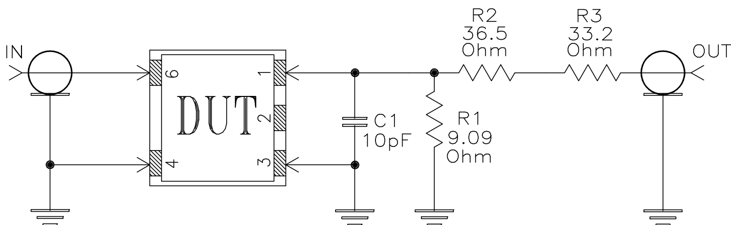
Schematic Diagram
