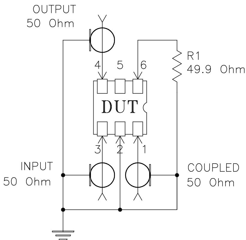
Schematic Diagram
