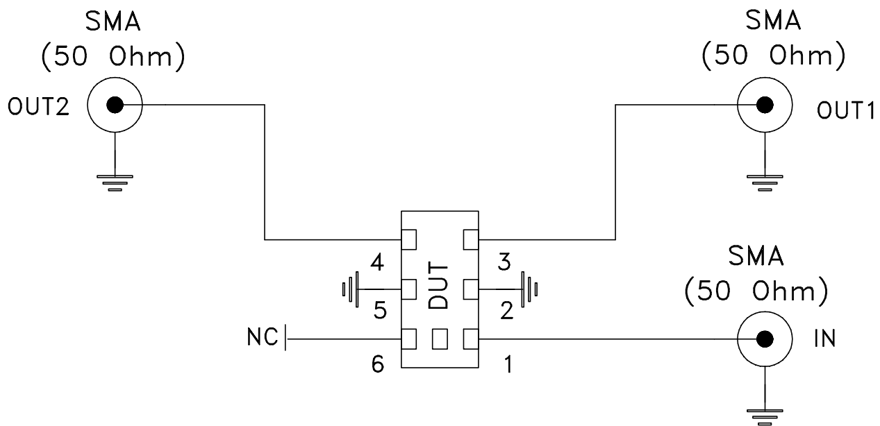
Schematic Diagram
