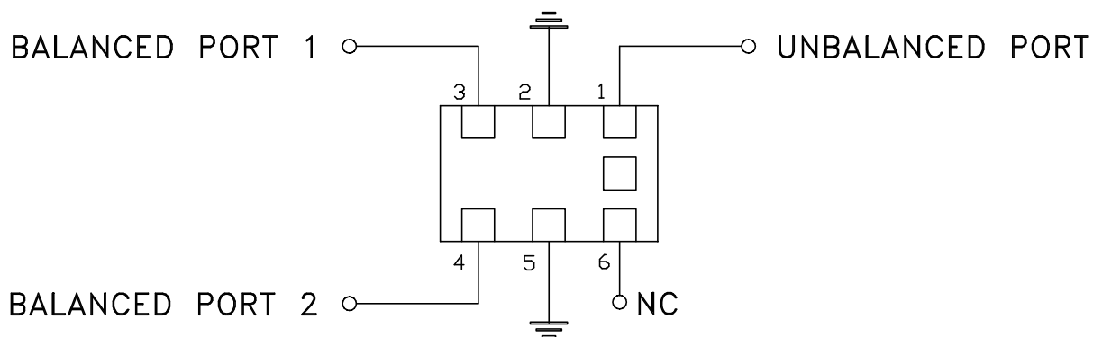
Schematic Diagram
