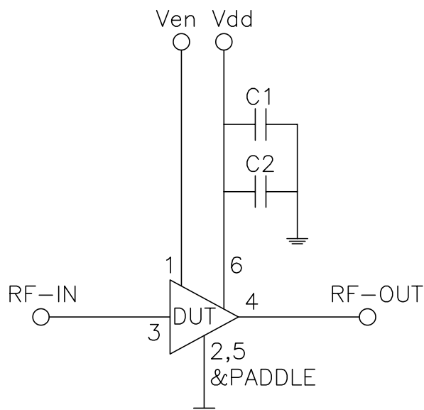
SCHEMATIC DIAGRAM
