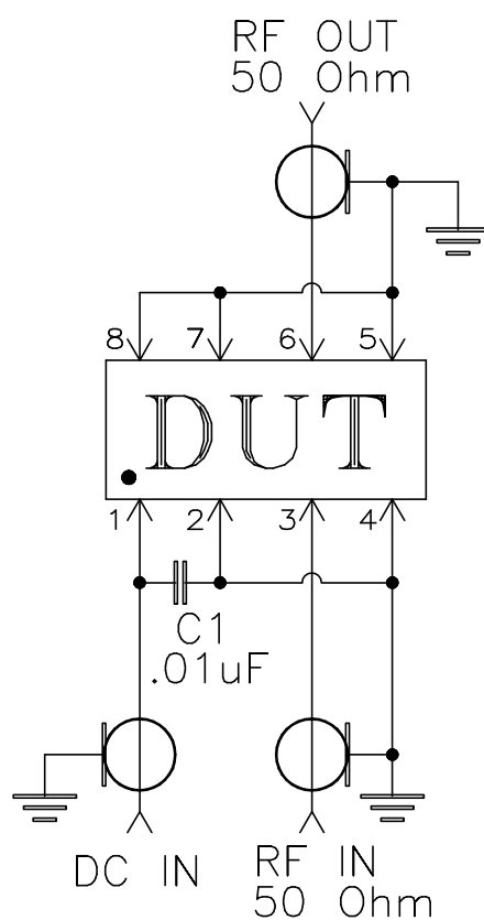
Schematic Diagram
