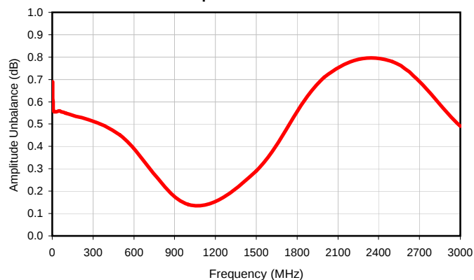
Amplitude Unbalance
