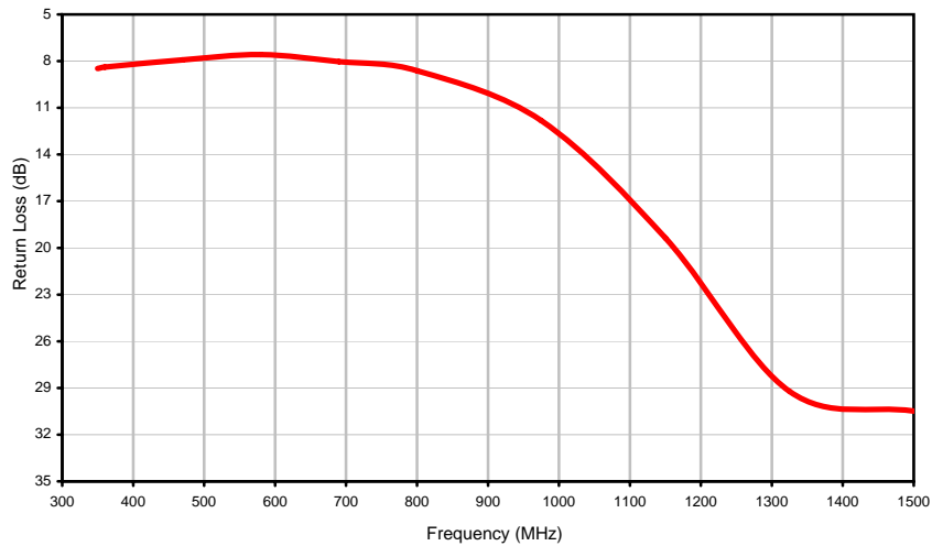
Return Loss
