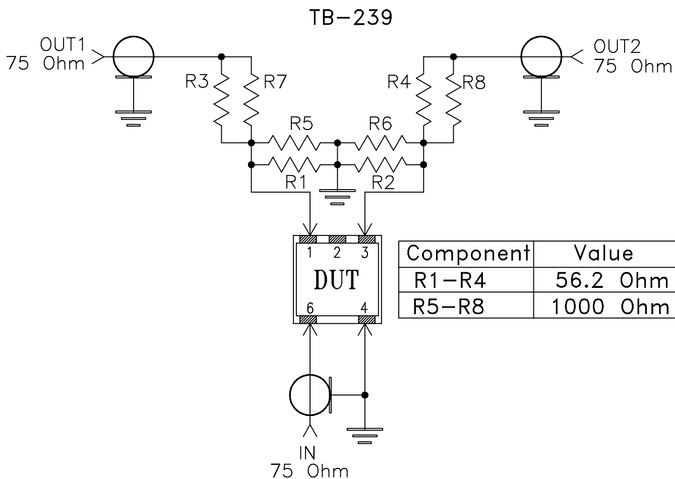
Schematic Diagram
