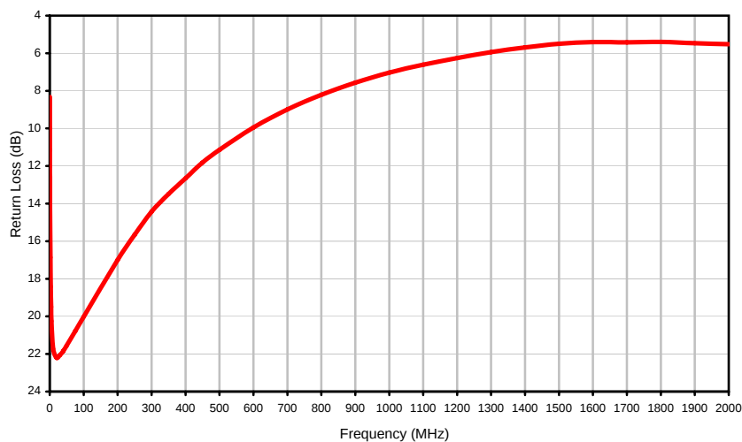
Return Loss
