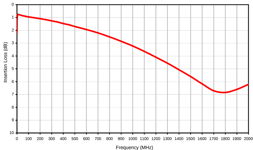
Insertion Loss
