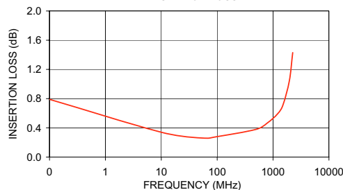
TC1.5-1MG2+ INSERTION LOSS
