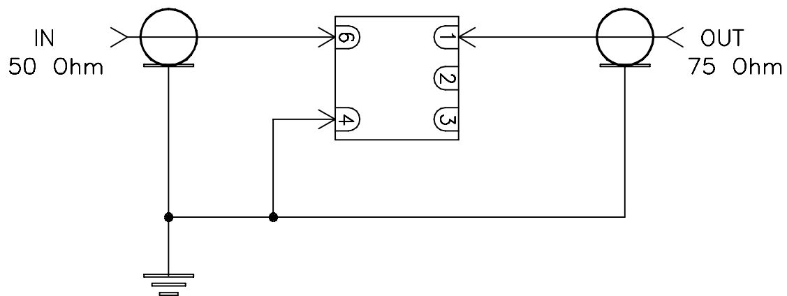
Schematic Diagram
