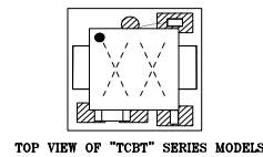
TOP VIEW OF "TCBT" SERIES MODELS
