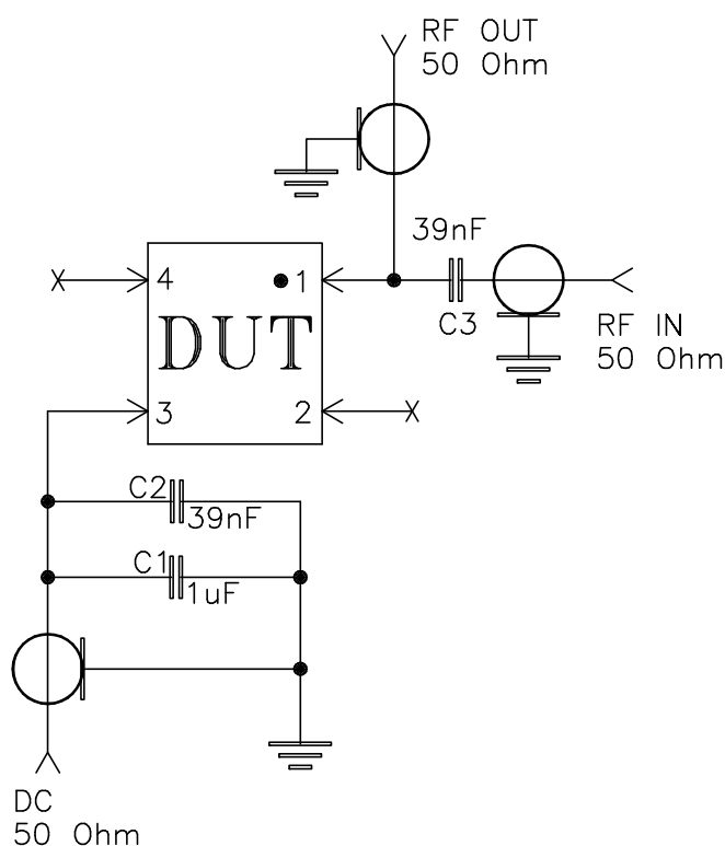
Schematic Diagram
