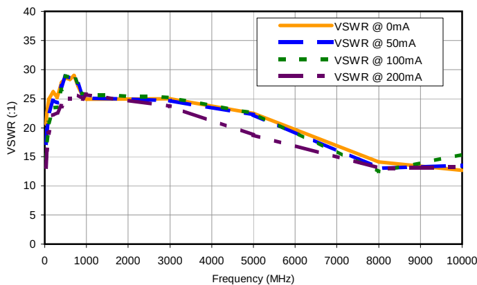
Return Loss vs. Frequency &amp; Current
