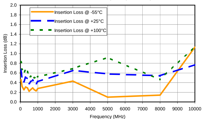
Insertion Loss vs. Frequency &amp; Temperature
