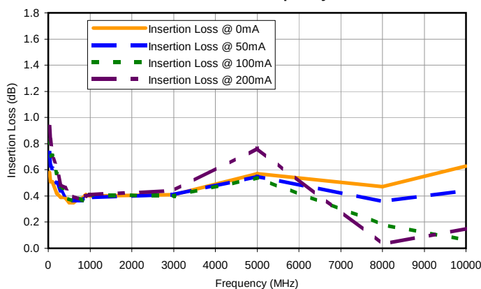
Insertion Loss vs. Frequency &amp; Current
