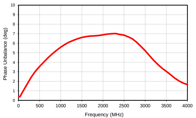
Phase Unbalance
