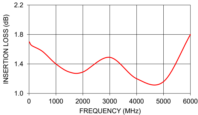
TCM1-63AX-2+ INSERTION LOSS
