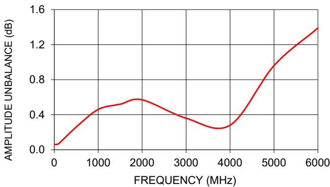
TCM1-63AX-2+ AMPLITUDE UNBALANCE
