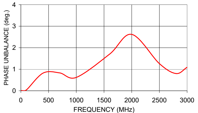
PHASE UNBALANCE
