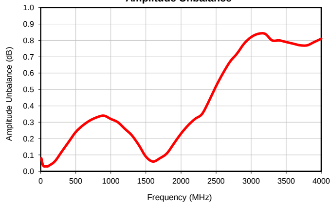
Amplitude Unbalance
