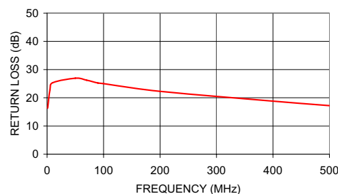
TCM3-1T INPUT RETURN LOSS
