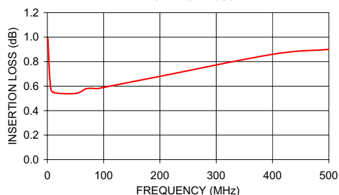
TCM3-1T INSERTION LOSS
