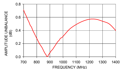
TCN2-14 AMPLITUDE UNBALANCE
