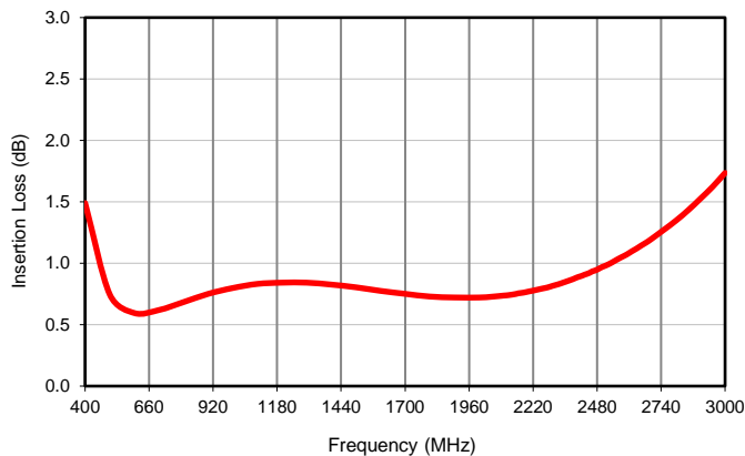
Insertion Loss
