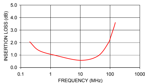
TMO-14-1+ INSERTION LOSS
