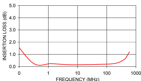
TMO-2-1+ INSERTION LOSS
