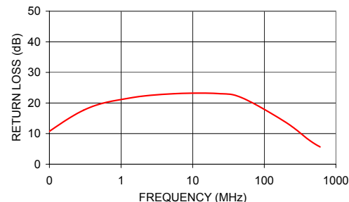
TMO-2-1+ INPUT RETURN LOSS
