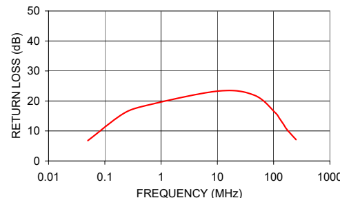
TMO-3-1T+ INPUT RETURN LOSS
