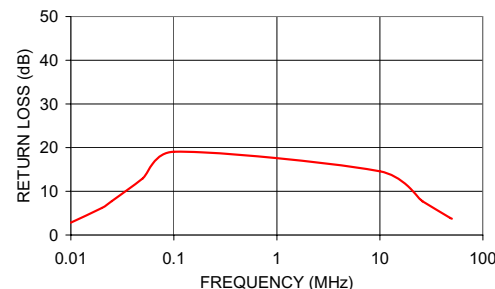
TT2.5-6 INPUT RETURN LOSS
