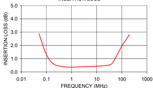
TT4-1-KK81 INSERTION LOSS
