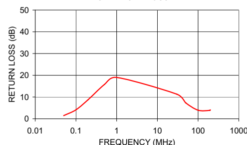
TT4-1-KK81 INPUT RETURN LOSS
