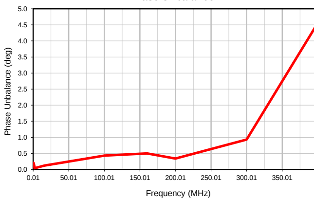
Phase Unbalance
