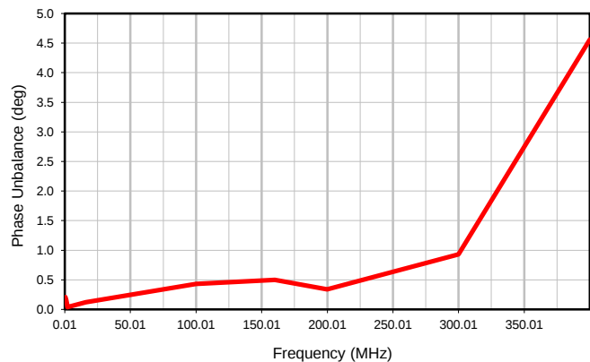
Phase Unbalance
