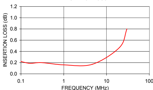
TTMO-25-1+ INSERTION LOSS
