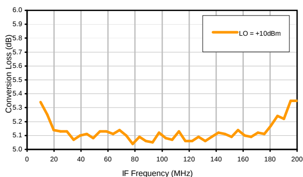
Conversion Loss vs. IF @ RF=210.1MHz
