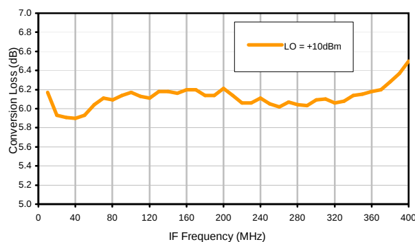
Conversion Loss vs. IF @ RF=410.1MHz
