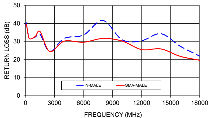
ULC-3FT-SMNM+ RETURN LOSS
