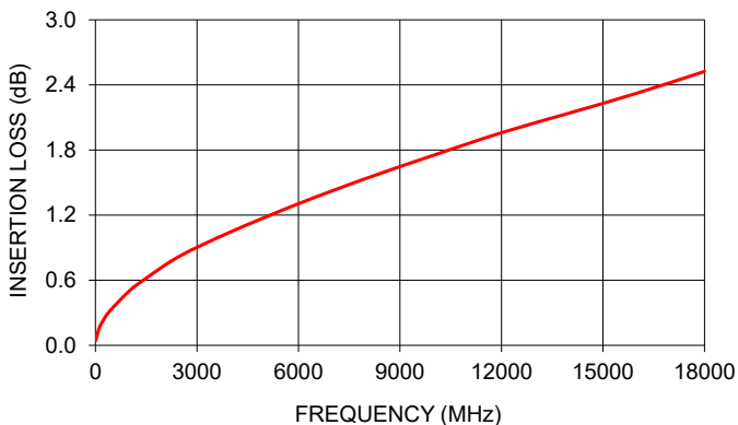
ULC-3FT-SMNM+ INSERTION LOSS
