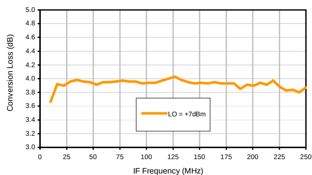
Conversion Loss vs. IF @ RF=260.1MHz
