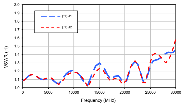
VSWR, Terminated Ports
