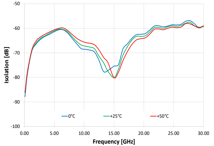
Isolation J1 to J2 (J1 Active)
