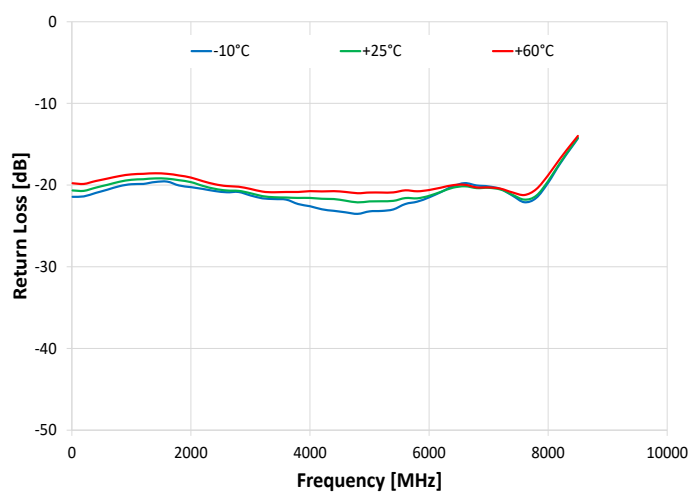
Return Loss @ 1 over Temperature (1 Active)
