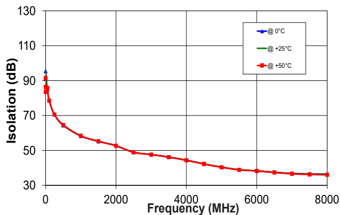
Com to Port Isolation over Temp.
