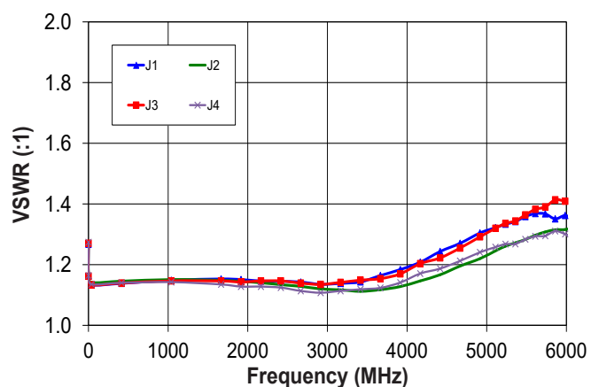
VSWR J1/2/3/4 Terminated Ports
