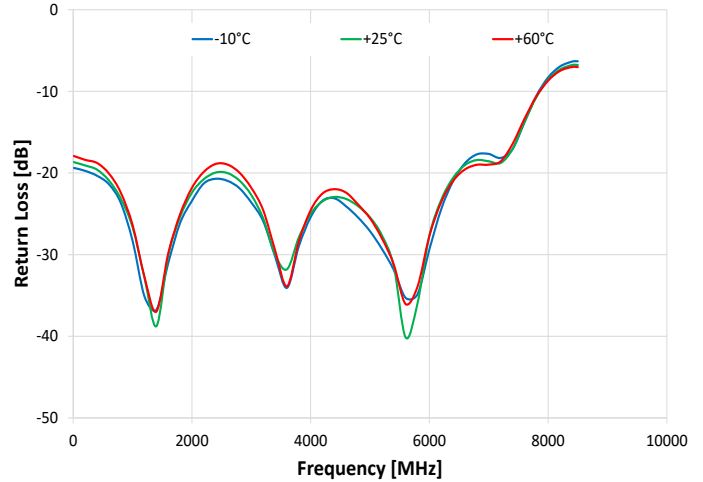
Return Loss @ J1 over Temperature (J1 Terminated)
