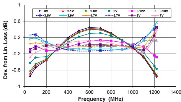
VAEQ-1220+ DEVIATION FROM LINEAR LOSS Vs. FREQUENCY OVER CONTROL VOLTAGES
