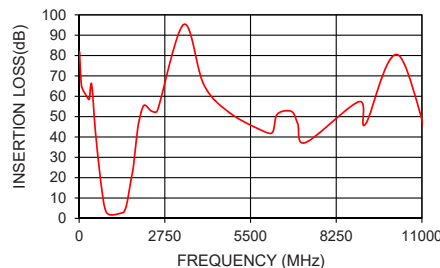
VBFZ-1065-S+ INSERTION LOSS
