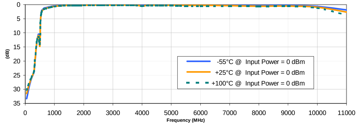
OUTPUT RETURN LOSS vs. TEMPERATURE
