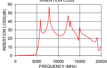
VLF - 3800+ INSERTION LOSS
