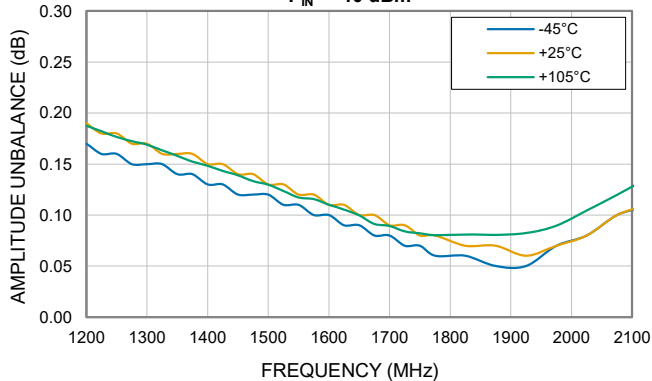
AMPLITUDE UNBALANCE vs TEMPERATURE, P IN = -10 dBm
