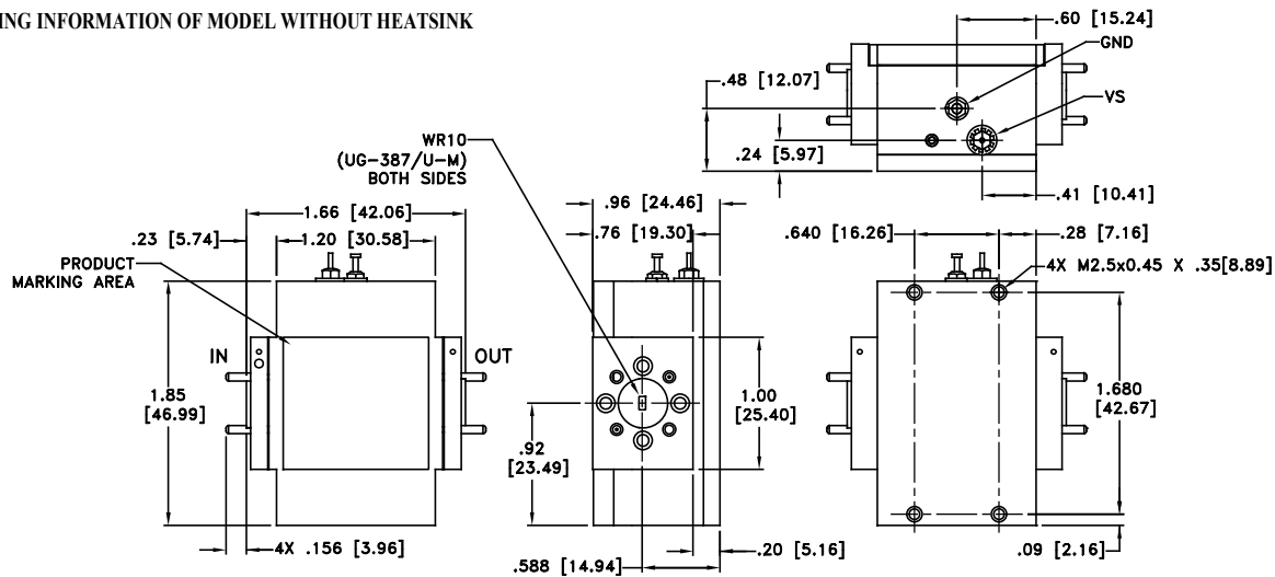
MOUNTING INFORMATION OF MODEL WITHOUT HEATSINK
