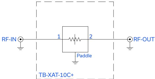
Figure 2. XAT-10+ Characterization and Application Circuit.
