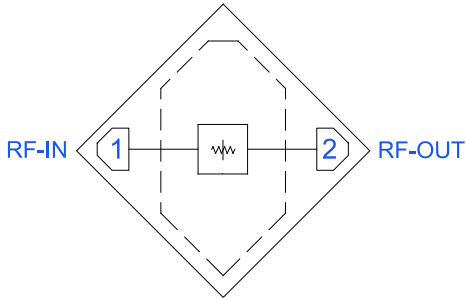
Figure 1. XAT-10+ Functional Diagram
