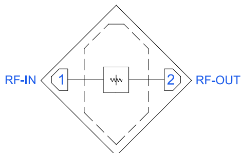
Figure 1. XAT-20+ Functional Diagram
