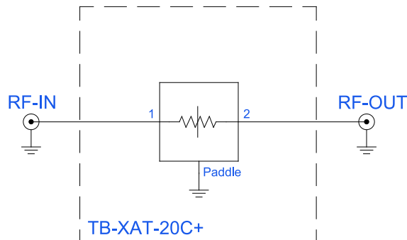
Figure 2. XAT-20+ Characterization and Application Circuit.
