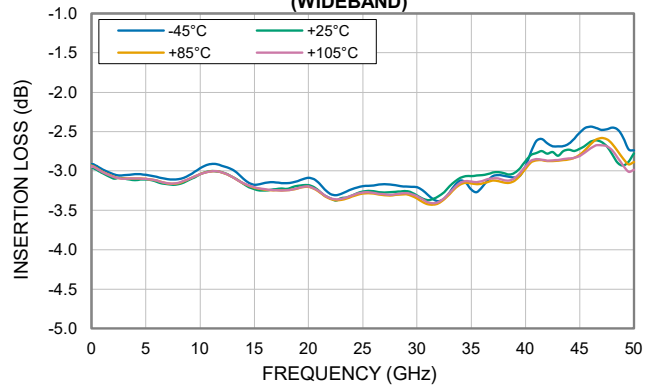
INSERTION LOSS vs. TEMPERATURE (WIDEBAND)
