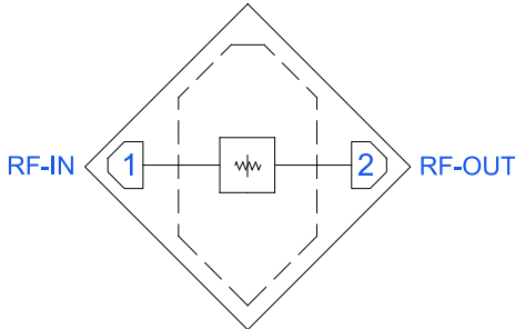
Figure 1. XAT-3+ Functional Diagram
