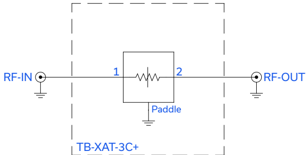
Figure 2. XAT-3+ Characterization and Application Circuit.
