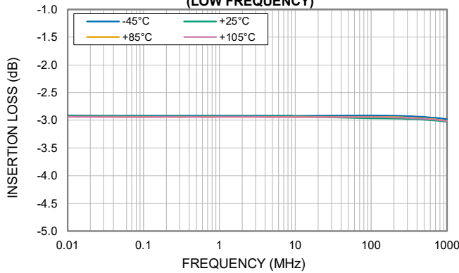
INSERTION LOSS vs. TEMPERATURE (LOW FREQUENCY)
