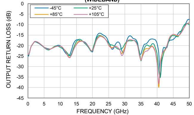
OUTPUT RETURN LOSS vs. TEMPERATURE (WIDEBAND)
