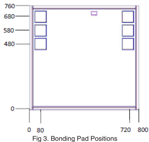
Fig 3. Bonding Pad Positions
