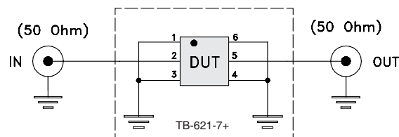
Fig 1. Block diagram of Test Circuit used for characterization, Test board TB-621-7+ Conditions: Attenuation, VSWR: Pin=-10 dBm
