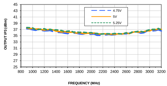
OUTPUT IP3 vs. FREQUENCY & DEVICE VOLTAGE OUTPUT POWER = 2.5 dBm/100W, Temperature = +25°C
