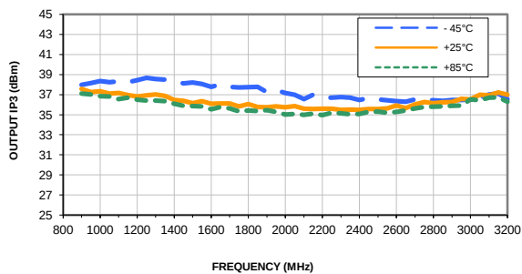
OUTPUT IP3 vs. FREQUENCY & TEMPERATURE OUTPUT POWER = 2.5 dBm/100W, Vd = 5.00V
