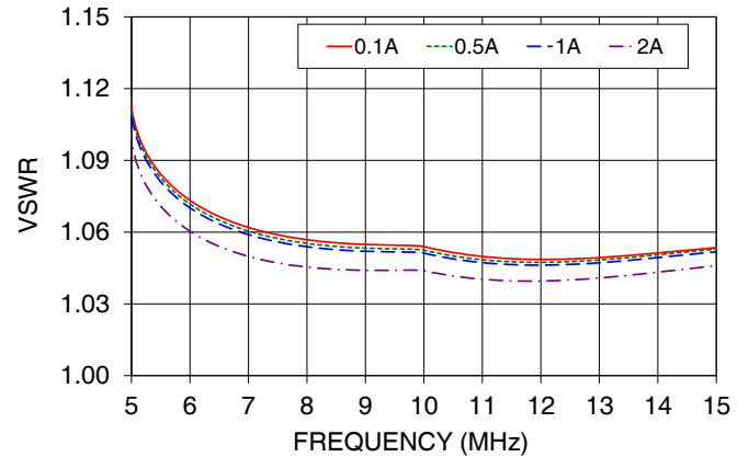
Z4BT-2R15G+ REF port VSWR ( P_{in} = 0\text{dBm} )
